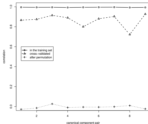
Figure 4 First nine canonical correlations. Canonical correlations in the training data set, in the validation data set and after permutations.
