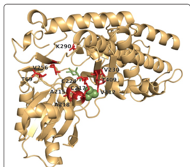
Figure 6 smHK residues with highest conz(k) -values. For smHK, H2rs predicted 10 residues with conz(k) -values \geq 2.0 and p -values \leq 10^{-11} , which are shown as red sticks. The ligand GLC is shown as green sticks and the SO 4 ion in the catalytic cleft as green balls.
