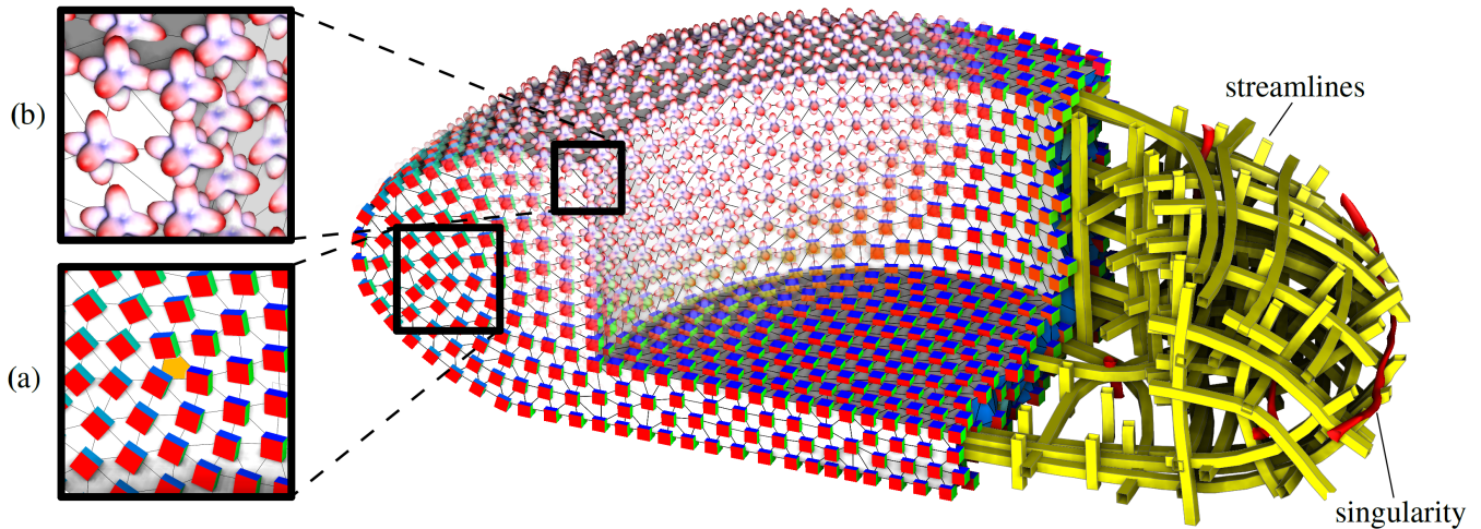
Figure 1: Our algorithm produces smooth frame fields in volumes. Frames (a) are represented by spherical harmonic functions (b), attached to each vertex of a tetrahedral mesh. Streamlines and singularities of the field are shown in yellow and red, respectively.
