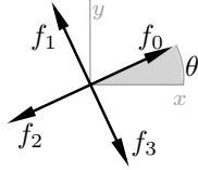
Figure 2: A 2D frame is a set of 4 vectors f_0, f_1, f_2, f_3 invariant under rotation by \pi/2 . Its angular representation is the rotation \theta between the global axis x and f_0 .
