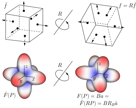
Figure 4: An arbitrary frame f corresponds to the reference frame \tilde{f} rotated by a 3 \times 3 matrix R . The graphs of the corresponding functions \tilde{F} and F are also rotated by R , and their coefficients vectors verify a = R_B \tilde{a} where R_B is a 9 \times 9 rotation matrix (derivation detailed in the supplemental material).
