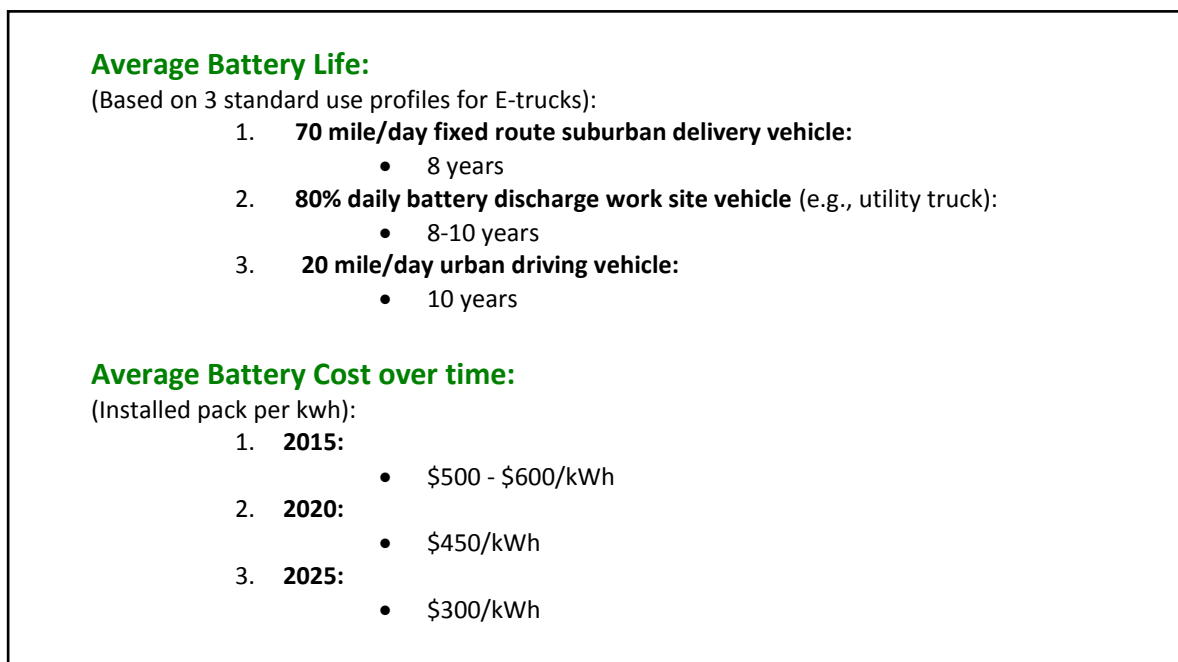
Figure 8: Expected battery pack life in common use profiles, and expected future pack costs
