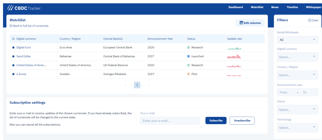
Figure 7: Watchlist
