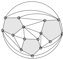
Figure 10: A plane topological graph in which any augmentation leaves \frac{2n}{5} vertices without meeting its parity constraints.
