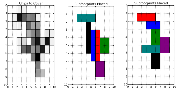
(a) Chips to cover. (b) Greedy solution. (c) Optimal MIP.
