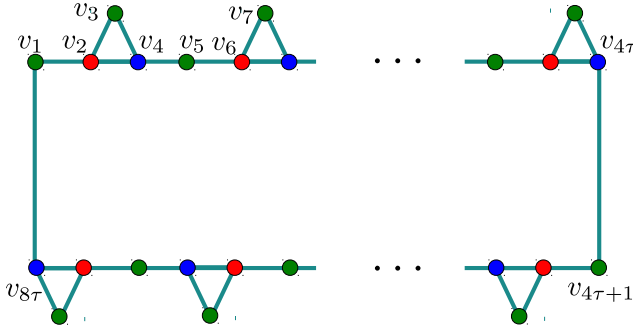
Figure 3: The graph G .
