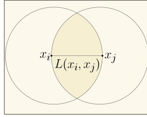
Figure 2: L(x_i, x_j)
