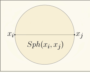
Figure 1: Sph(x_i, x_j)
