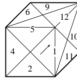
Figure 4: Adjacency relationship of the squares on the cube of size \sqrt{2} \times \sqrt{2} \times \sqrt{2} .
