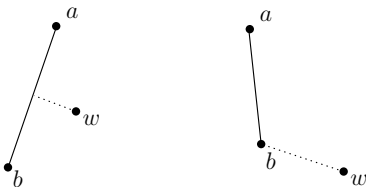
Figure 2: \|(a, b) - w\| is the minimum distance between w and any point on (a, b) .
