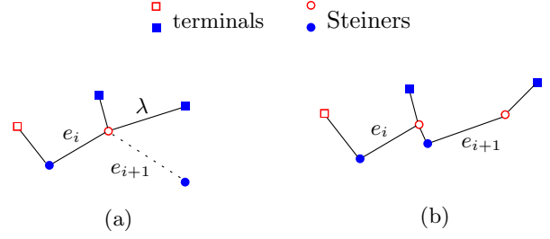
Figure 1: The optimal full bichromatic Steiner tree is obtained (a) from \mathcal{T}_i , when |e_i| < \lambda < |e_{i+1}| and (b) from \mathcal{T}_{i+1} , when \lambda = |e_{i+1}| .
