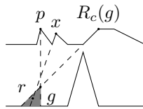
Figure 3: A point r is g -ceiling-dominated.
