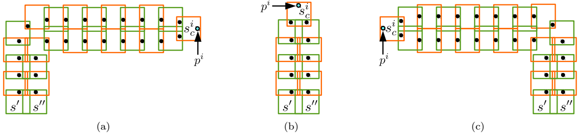
Figure 3: (a) A left chain. (b) A middle chain. (c) A right chain.
