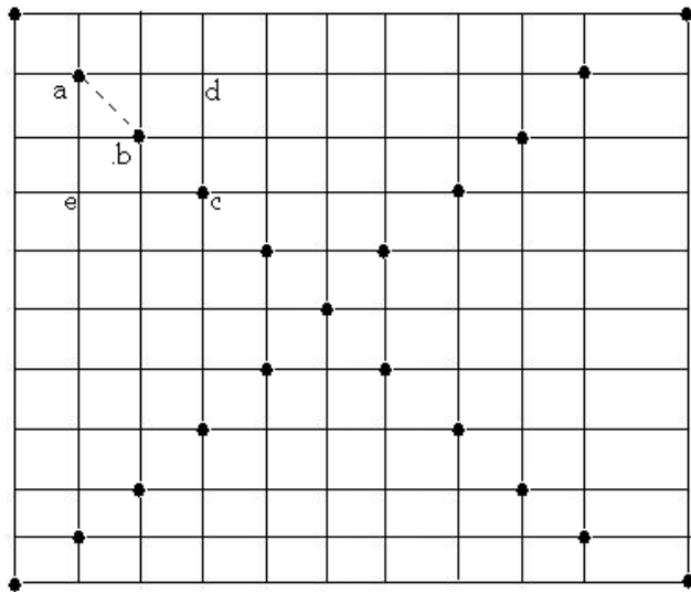
Figure 1. The rectangular surveillance zone with the sensors shown as circles placed along the two zone diagonals at the corners of the cells. The sensors have a radius of vision equal to the diagonal of the cell
