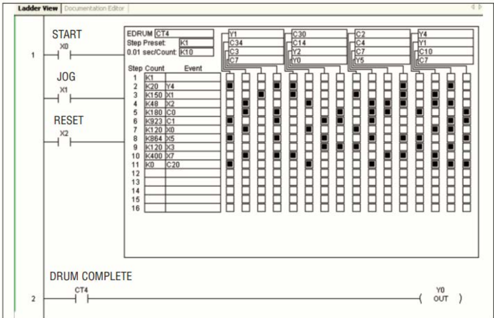
DirectSOFT Display
