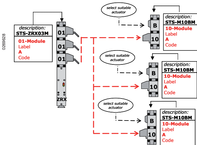
Example: ZRH-3GATE-SET
