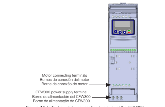
Figure A4: Indication of the connecting terminals of the CFW300 Figura A4: Indicación de los bornes de conexión del CFW300 Figura A4: Indicação dos bornes de conexão do CFW300
