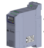
(c) Retract the lower snaps of the filter set into the CFW300 base (c) Retraer as trabas inferiores del conjunto filtro en la base del CFW300 (c) Recolha as trabas inferiores do conjunto filtro na base do CFW300
