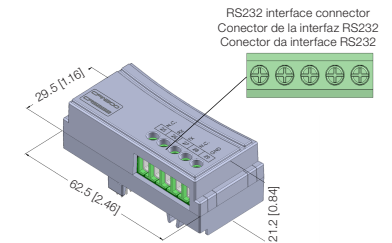
Figure A2: CFW300-CRS232 dimensions in mm [in] and connectors location
