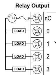
Relay Output Wiring Diagram
