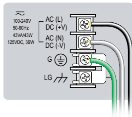
100-240 VAC, 125VDC
