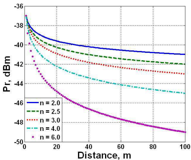
Fig. 10. Effects of Path Loss Exponent (Pu, 2009).
