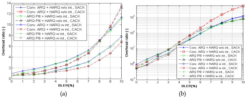
Fig. 16. ARQ & HARQ Overhead vs. BLER for ARQ_Block_Size = 16 B, PDU Size = 16, Size of user data = 1024 B/frame, 2 HARQ retrans., HARQ Type: IR, 1 hop (a) / 3 hops (b)
