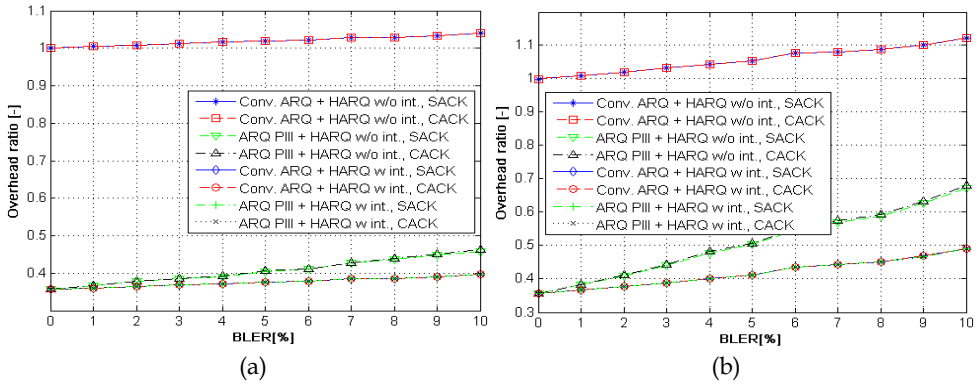
Fig. 9. ARQ & HARQ Overhead vs. BLER for ARQ_Block_Size = 1024 B, PDU Size = 1, Size of user data = 1024 B/frame, 2 HARQ retrans., HARQ Type: CC, 1 hop (a) / 3 hops (b)
