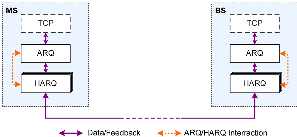
Fig. 3. Principle of ARQ and HARQ cooperation
