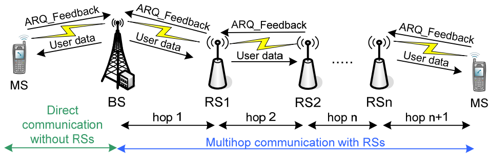
Fig. 4. Link level simulation scenario
