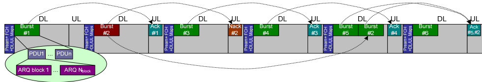
Fig. 1. Principle of conventional ARQ
