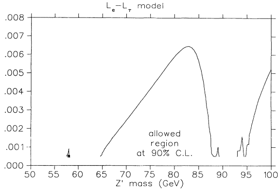
FIG. 3. The allowed region at 90% C.L. in (g'_2, M_{Z'_2}) space for the gauged L_e-L_\tau model.
