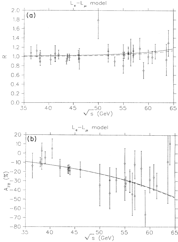
FIG. 6. (a) R_\mu corresponding to the maximum allowed coupling constant case in the TRISTAN/LEP window for the gauged L_e-L_\mu model (solid line), compared with the MSM best fit (dashed line). (b) A_{FB}^\mu in the TRISTAN region corresponding to the maximum allowed coupling constant case in the TRISTAN/LEP window for the gauged L_e-L_\mu model (solid line), compared with the MSM best fit (dashed line).
