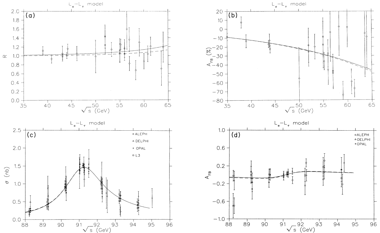
FIG. 5. (a) R_\tau corresponding to the maximum allowed coupling constant case in the TRISTAN/LEP window for the gauged L_e-L_\tau model (solid line), compared with the MSM best fit (dashed line). (b) A_{FB}^\tau for the TRISTAN region corresponding to the maximum allowed coupling constant case in the TRISTAN/LEP window for the gauged L_e-L_\tau model (solid line), compared with the MSM best fit (dashed line). (c) Z line shape corresponding to the maximum allowed coupling constant case in the TRISTAN/LEP window for the gauged L_e-L_\tau model (solid line), compared with the MSM best fit (dashed line). (d) A_{FB}^\tau in the LEP region corresponding to the maximum allowed coupling constant case in the TRISTAN/LEP window for the gauged L_e-L_\tau model (solid line), compared with the MSM best fit (dashed line).
