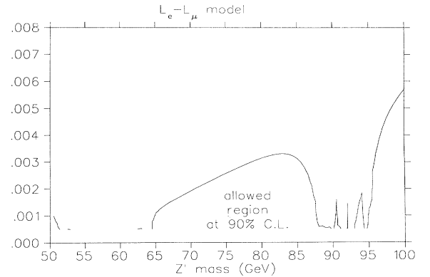
FIG. 2. The allowed region at 90% C.L. in (g'_i, M_{Z'_i}) space for the gauged L_e - L_\mu model.
