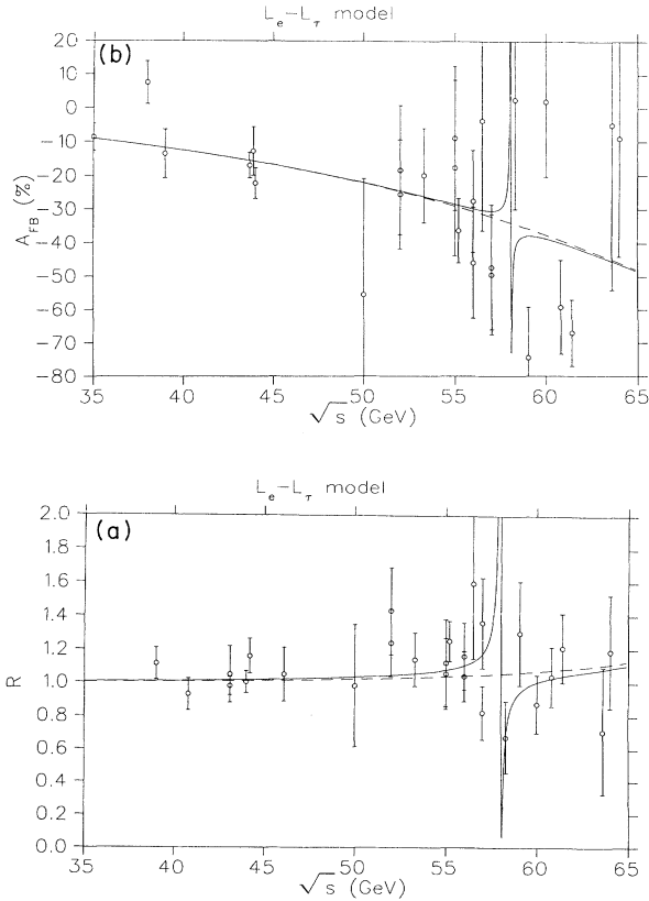
FIG. 4. (a) The best-fit point contribution to R_\tau for the gauged L_e-L_\tau model (solid line), compared with the MSM best fit (dashed line). (b) The best-fit point contribution to A_{FB}^\tau in the TRISTAN region for the gauged L_e-L_\tau model (solid line), compared with the MSM best fit (dashed line).
