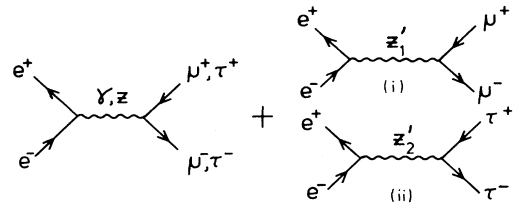
FIG. 1. Feynman diagrams showing the contributions of \gamma, Z , and Z'_{1,2} to e^+e^- \rightarrow (i) \mu^+\mu^- , (ii) \tau^+\tau^- .
