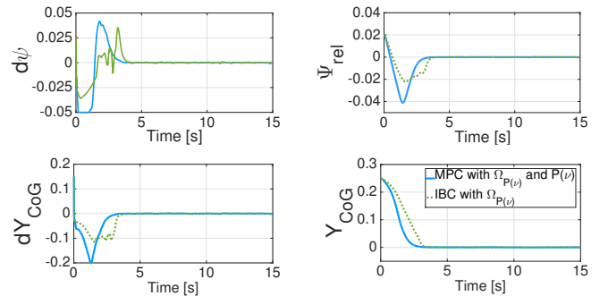
Fig. 3: States trajectories
