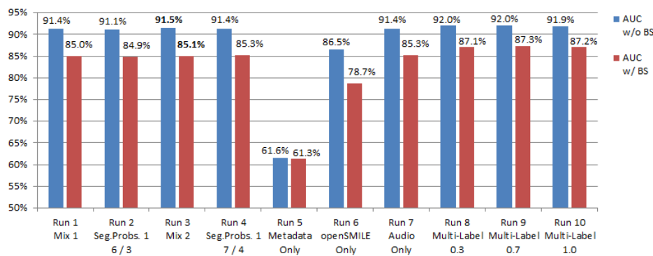
Fig. 5. Area Under the Curve (AUC) of Runs
