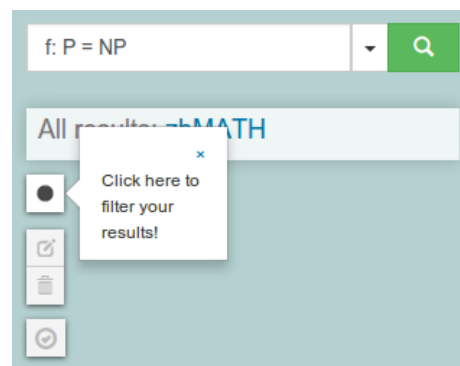
Fig. 7: Filtering toolbar.
