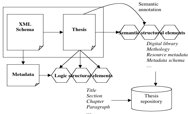
Fig. 3. Combination of logical and semantic structural elements
