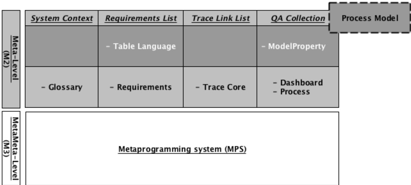
Fig. 1: A language stack for gathering software requirements
