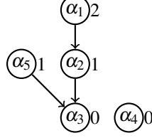
Figure 3. \top\perp^* -AD of B_1 with the height metric to the right of each atom
