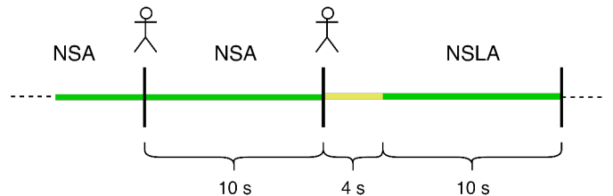
Fig. 7. Possible differences of simulation steps between actions.
