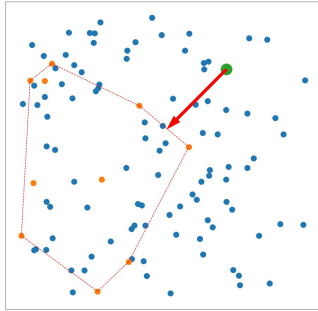
Figure 1: Visualization of Latent Convex Hull. Unexpectedness is defined as the distance between new item and latent convex hull generated by all consumed items.
