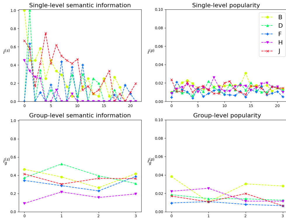
Figure 1: Variations computed using the personalized recommendation lists created starting from the seed tracks B, D, F, H, J. Results shown are obtained with the single level model described in Section 3.1.1 (semantic information (top left), popularity (top right)) and group level model described in Section 3.1.2 (semantic information (bottom left), popularity (bottom right)).
