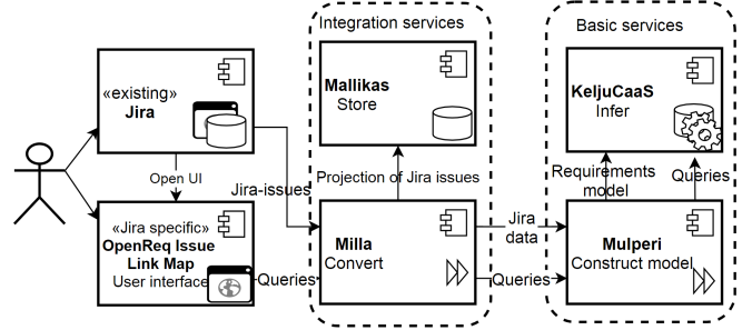
Figure 1. The architecture of the system.
