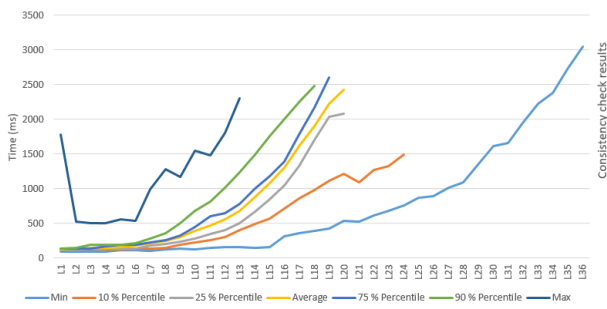
Figure 4. Time for consistency check using 3s timeout. Max at depth 1 is probably an error.
