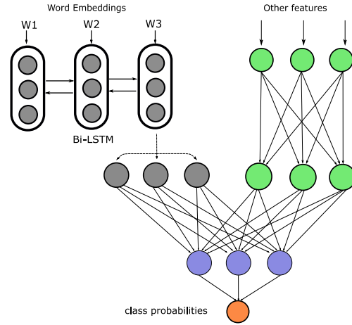
Fig. 1. The Bidirectional LSTM-based model used in our second submission.
