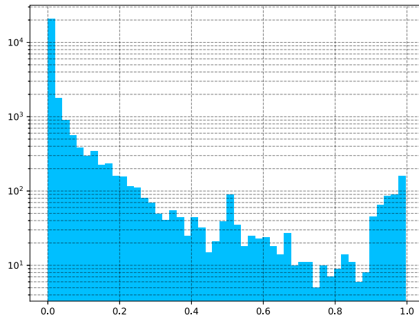
Fig. 4: Histogram of normalized bounding box sizes, where 1.0 corresponds to an area of 512x512. Figure 4 shows the histogram of the bounding boxes. According to this figure, most of the bounding boxes are located in the region where bounding boxes are smaller than the median area (256x512); therefore, 12, 25, and 80-pixel sizes for both width and height have been used for smaller boxes. For the mid-size and larger bounding boxes, 256 and 384 pixels have been chosen respectively. Each anchor box size [12, 25, 80, 256, 384] was mapped to the corresponding feature map layer in [P_2, P_3, P_4, P_5, P_6] respectively where P_n is the n^{th} feature map layer. Three different aspect ratios (width/height): 0.5, 1, and 2, were used for each anchor box.
