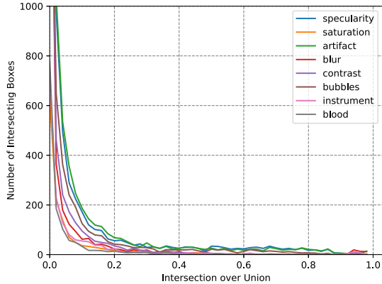
Fig. 2: IoU histogram of each class with the other seven classes. Vertical axis is clipped to provide better visualization. A threshold of 0.4 IoU is applied to the output of the ensemble model. In the remainder of this section, we describe these steps in more detail.
