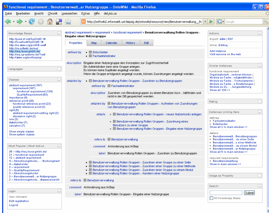
Figure 5: Functional requirement instance related to user roles and access control of the e-government application
