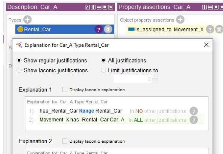
Fig. 1. Protégé display of inferred triples. One is indicated as inferred with a yellow background. An explanation box shows for another inferred triple.
