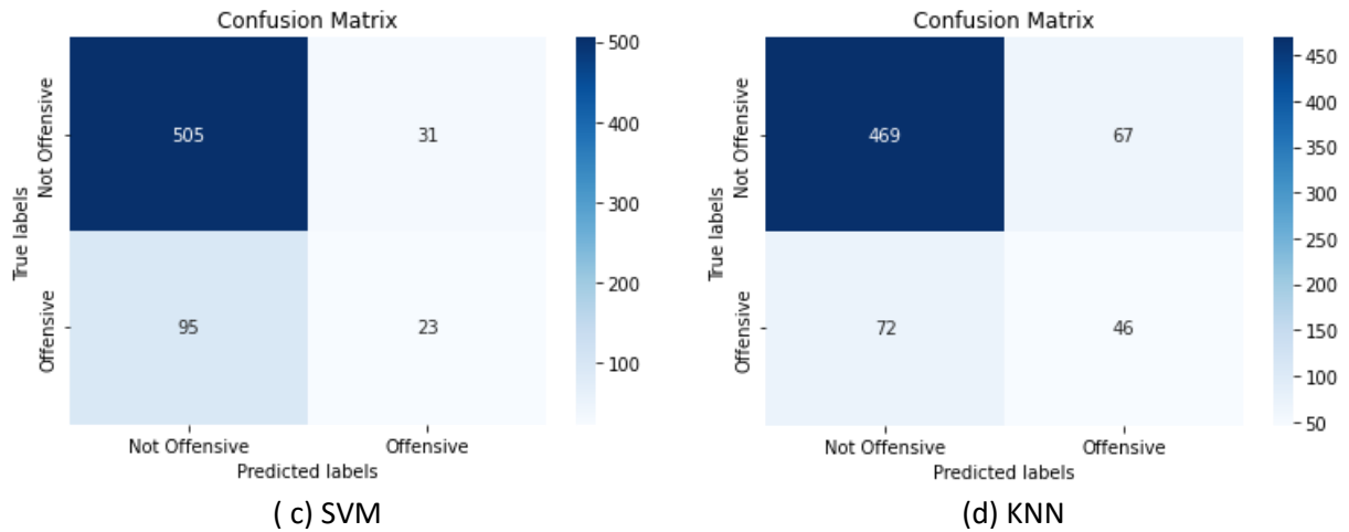
Figure 1. Confusion Matrix
