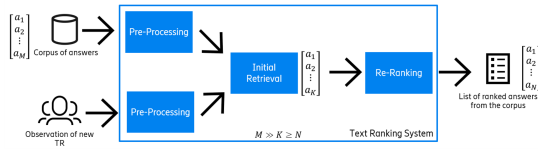
Figure 3: BERTicsson architecture.
