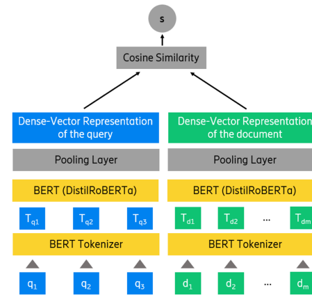
Figure 5: Sentence-BERT architecture.
