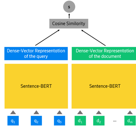
Figure 4: The IR stage architecture.
