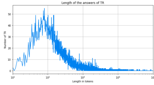
Figure 8: The Answer field.
