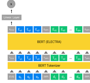
Figure 6: The RR stage and the monoBERT model.
