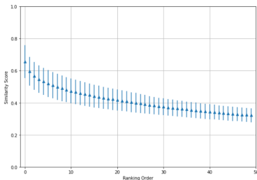
Figure 11: Mean and standard deviation of the cosine similarity scores in the IR along with the ranked list length.
