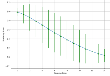
Figure 12: Mean and standard deviation of the similarity scores in the RR stage along the ranked list.
