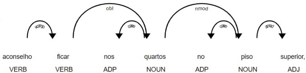
Figure 4: Example of a Dependency Tree
