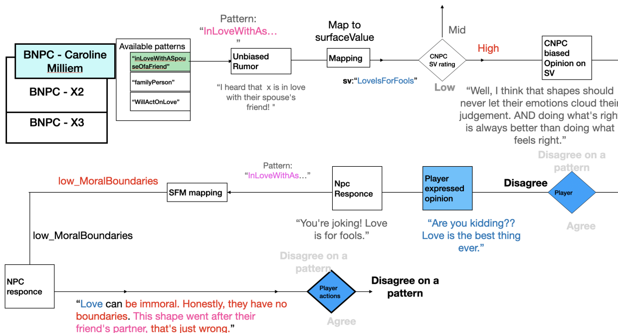
Figure 3: Deep value conversation loop - player disagrees with high surface value
