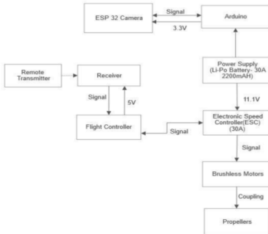
Figure 5: Block diagram
