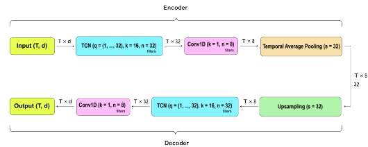
Figure 2: The architecture of the TCN-based autoencoder (TCN-AE)
