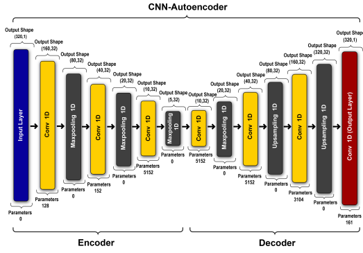
Figure 1: The architecture of the CNN-based autoencoder (CNN-AE)
