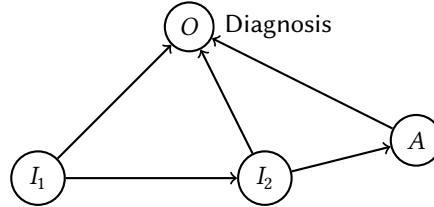
Figure 2: Graph of a small diagnostic BN.
