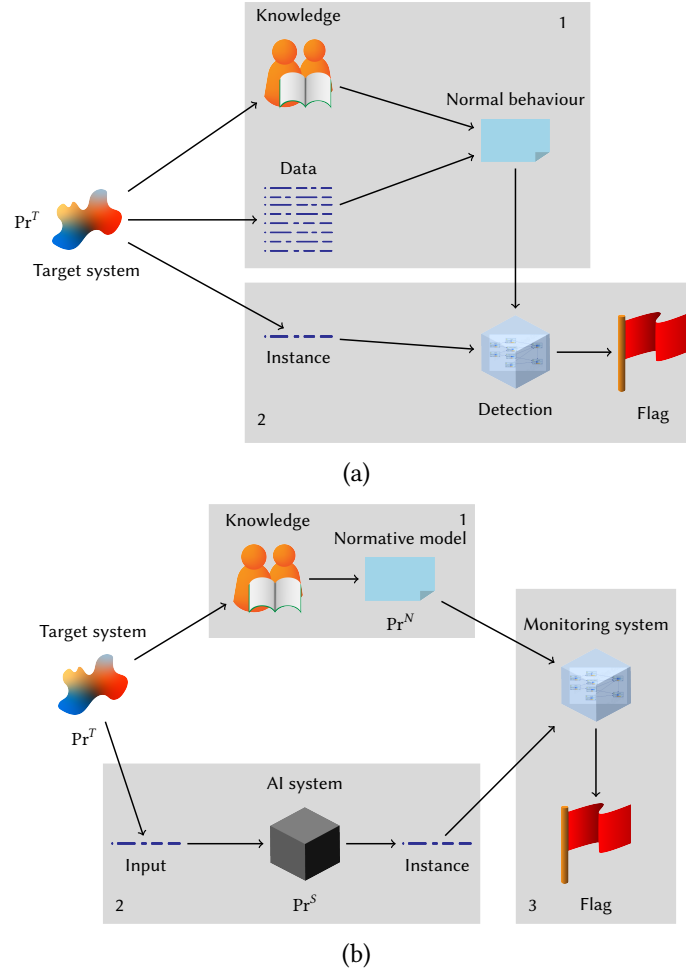
Figure 1: Overview of (a) Anomaly Detection with step 1 modelling normal behaviour and step 2 detecting anomalies and of (b) normative monitoring setting with step 1 constructing the normative model, step 2 running the AI system and step 3 monitoring an input-output pair.
