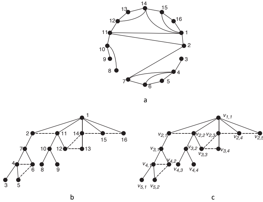
Figure 2: An outerplanar graph and its OBFT. (Figure from [6].)
