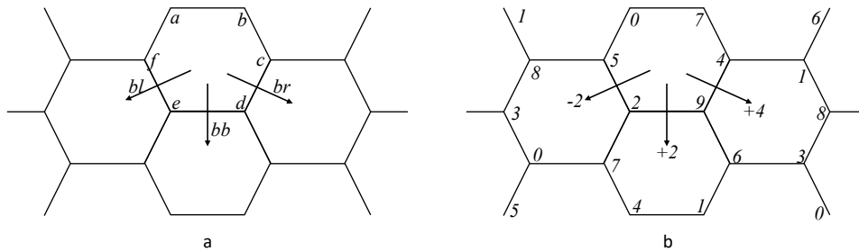
Figure 1: a. A portion of the hexagonal grid with the names associated with some of its nodes; b. L(3, 2, 1) -labeling of a portion of the hexagonal grid.
