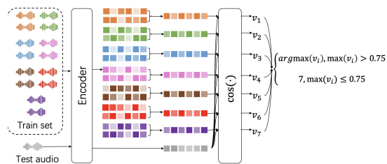
Figure 1: The implement pipeline of our proposed Center-based Maximum Similarity Method
