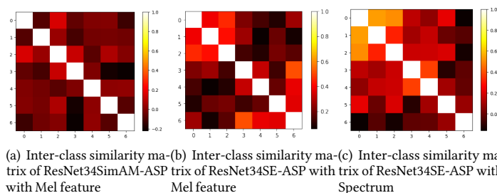
Figure 5: Inter-class similarity matrix for different system
