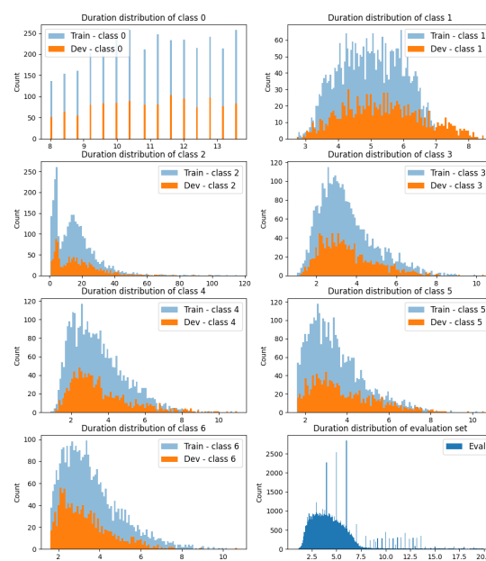
Figure 2: Distribution of audio durations in the train, development and evaluation set. The evaluation set is focusing on audio samples that are 20 seconds or less for ease of comparison.
