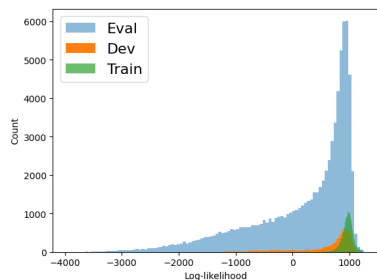
Figure 3: Distribution of log-likelihoods for all embeddings of the three sets. The higher the score, the higher the likelihood that the sample is from the same distribution as the training set.
