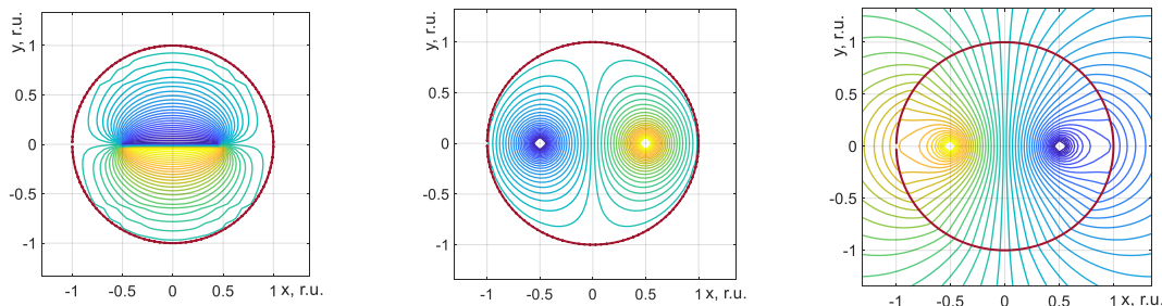
Figure 5: Flux lines (left) and equipotentials of current field in the insulated ladle (middle) and a non-metallic ladle (right) in the 2-electrode system
