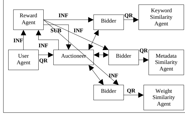
Fig. 2. Market-Based Recommender
