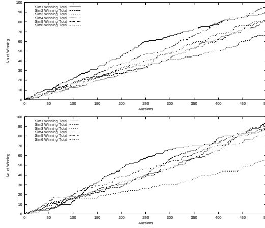
Fig. 6. Number of Wins ( x = 10\% , Y = 5\% , Z = 5\% )
