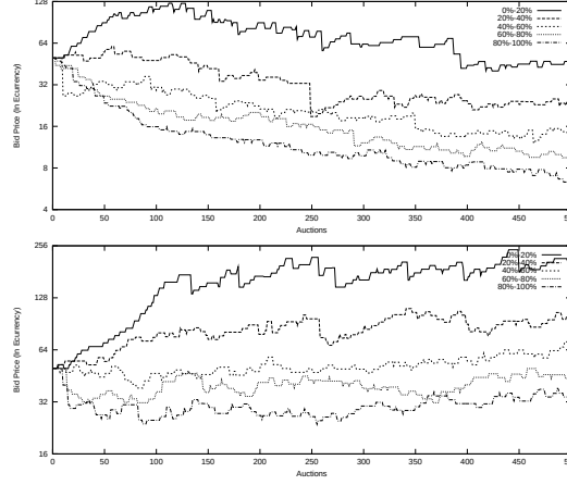
Fig. 5. Bid Price ( x = 10\% , Y = 5\% , Z = 5\% )
