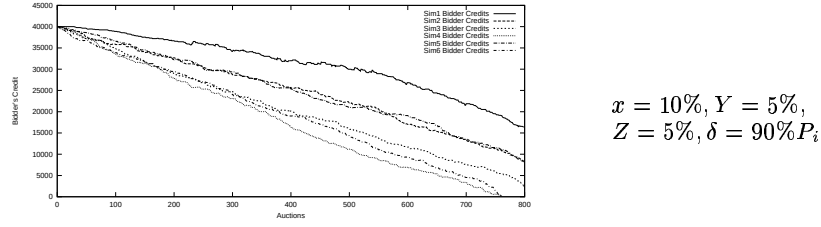
Fig. 8. Rational Bidder against Random Bidders
