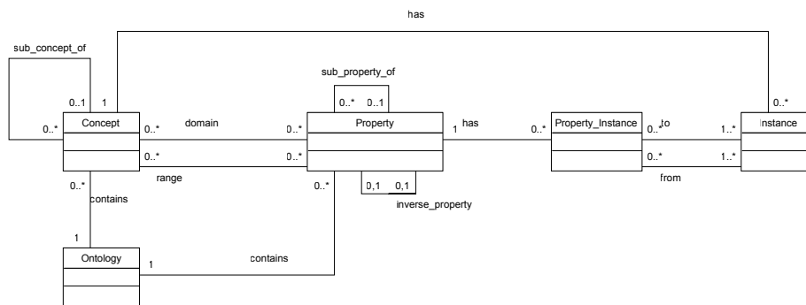
Fig. 4. Database schema for ontology
