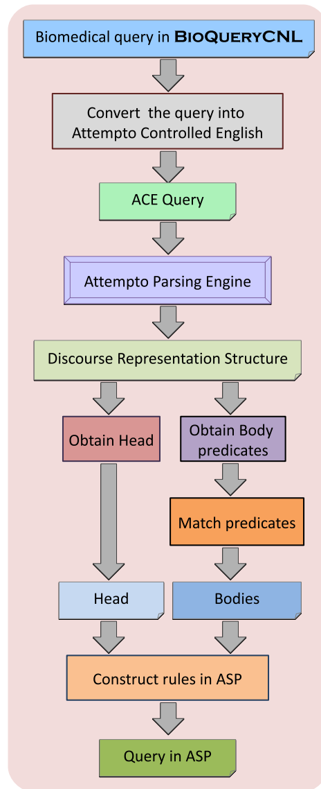
Fig. 1. Transforming a query in BIOQUERCNL into an ASP program.
