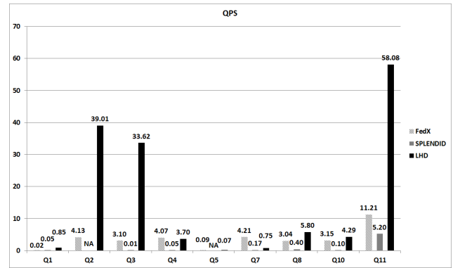
Figure 4: QPS of the three engines per query. NA means time out.
