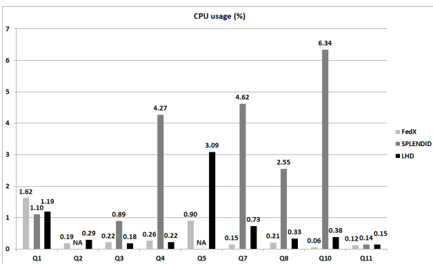
Figure 7: CPU usage of the three engines per query. NA means time out.
