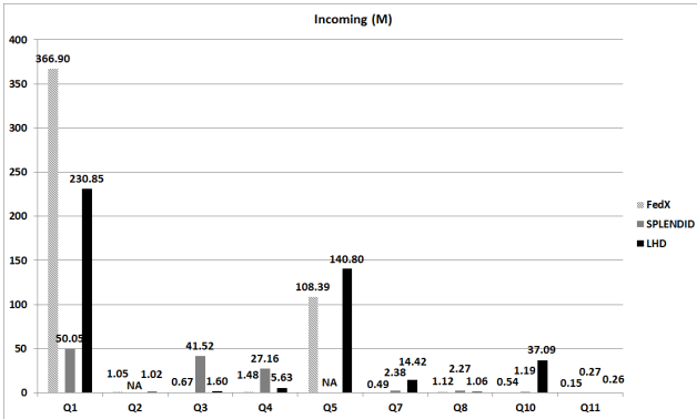
Figure 6: Incoming data of the three engines per query. NA means time out.
