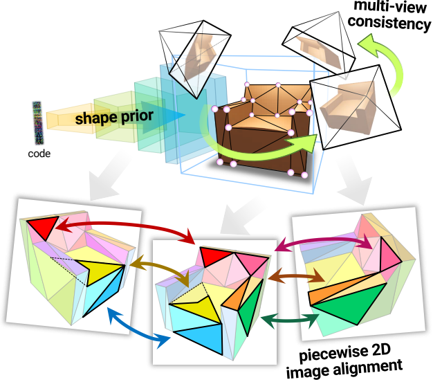
Figure 2: Overview. We perform 3D mesh reconstruction via piecewise image alignment of triangles to achieve per-triangle visibility-aware photometric consistency across multiple views, with mesh vertices optimized over the latent code of a shape prior learned by deep neural networks.
