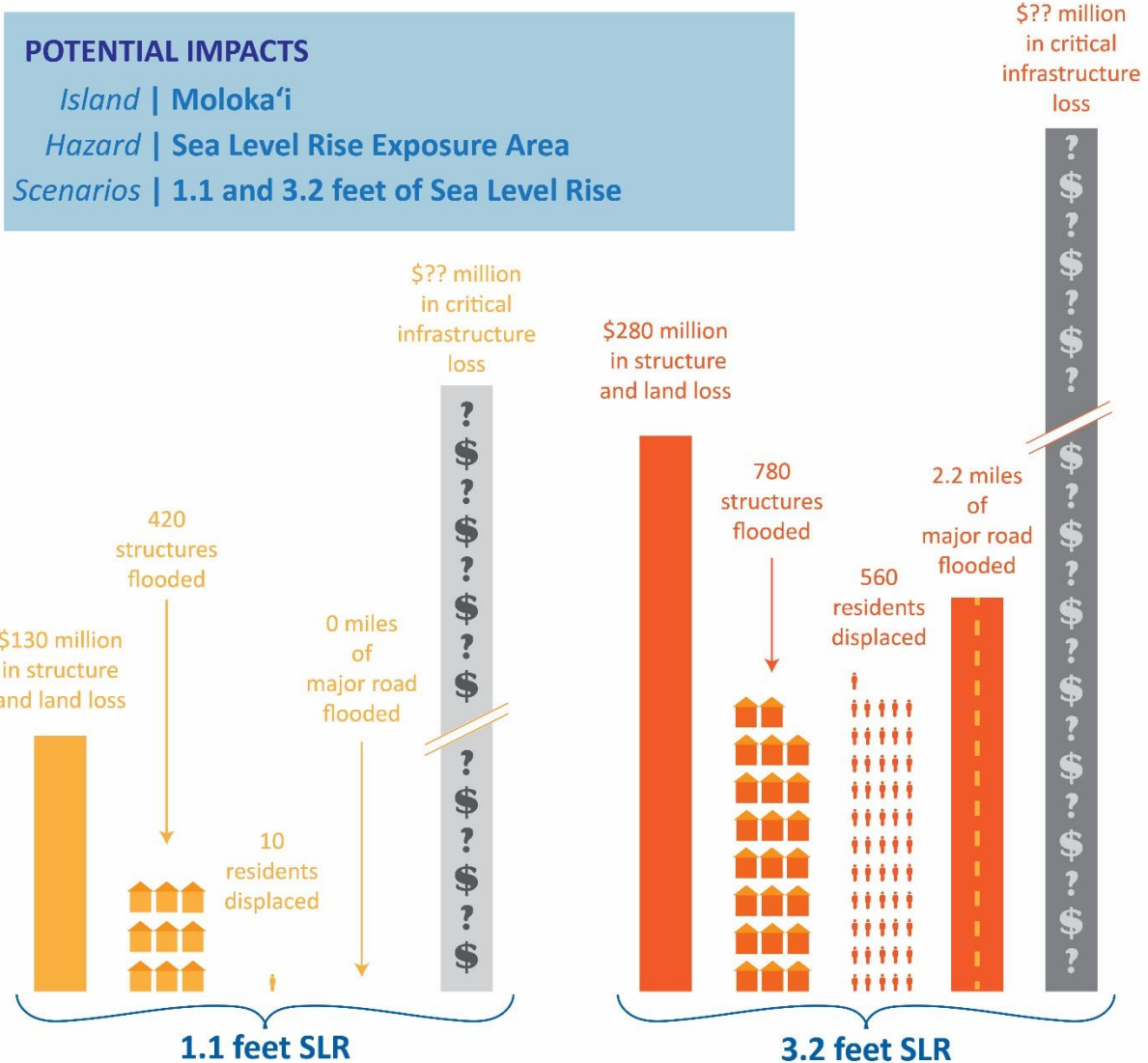
Figure 74. Summary of potential impacts in the SLR-XA with 1.1 feet and 3.2 feet of sea level rise on Moloka'i
