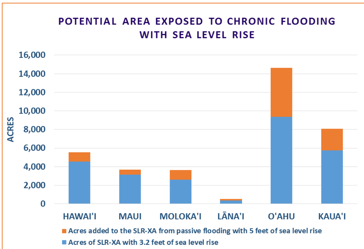
Figure 36. Potential additional area of chronic flooding with 5 feet of sea level rise
