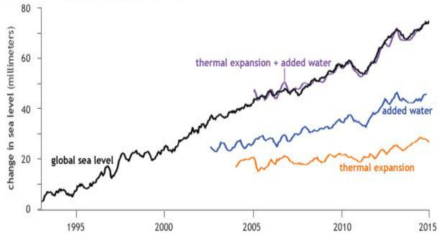
Figure 10. Contribution of thermal expansion and added water from glacier and ice sheet melting to sea level rise (Thompson et al. 2017)
