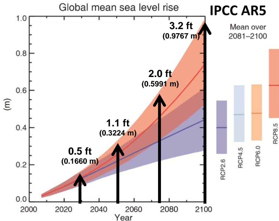
Projected rate of global sea level rise under different GHG scenarios (IPCC 2014)
