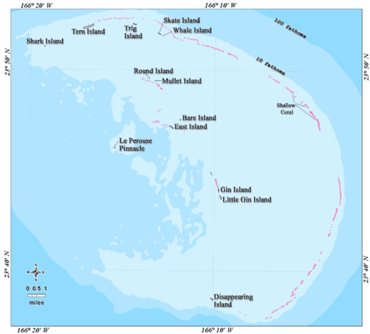
Figure 130. Islands and reef areas of French Frigate Shoals in the Northwestern Hawaiian Islands
