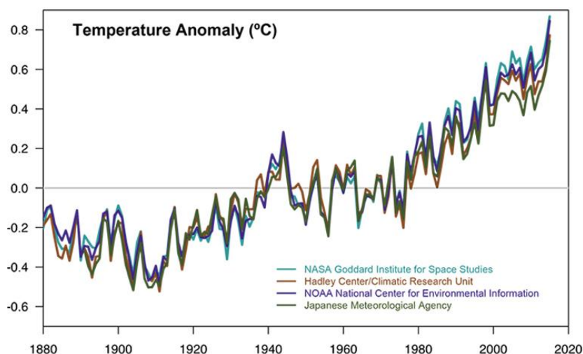
Figure 6. Global atmospheric temperature anomalies (NASA)
