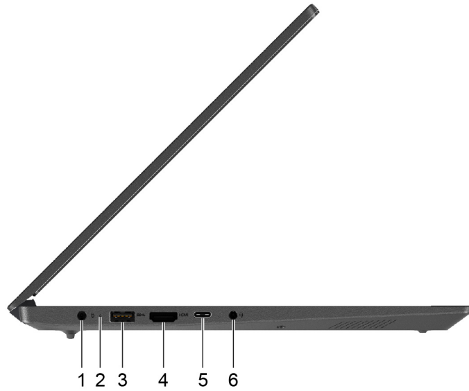
Figure 7. Left-side view—15-inch models
