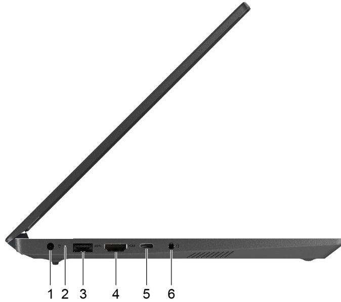
Figure 6. Left-side view—14-inch models
