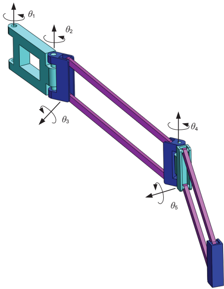
Fig. 5. The kinematic model of the exoskeleton (Type-II).
