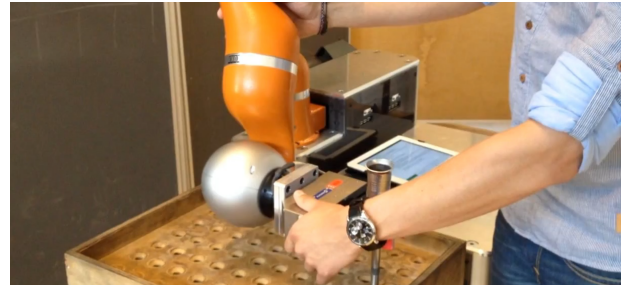
Fig. 6: Fotograf of an operator interacting with the manipulator and piloting it to a coordinate.
