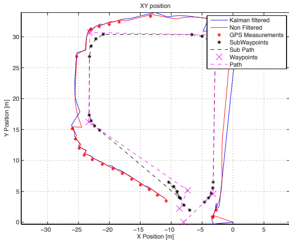
Fig. 4. Test 1 of the control and position estimation. The test was performed in the Klingenberg Pond at Aalborg University. As seen on the figure, the ship loses GPS signals due to the surroundings, but are still able to navigate the track.
