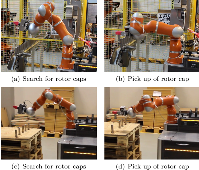
Fig. 3. Execution of vision pick skill. The robot captures images while moving in (a). The images are send to the quality control system shown in Figure 1, and whenever a rotor cap is detected, the robot picks it up, as shown in (b). Figures (c) and (d) show the same skill executed at a different location.
