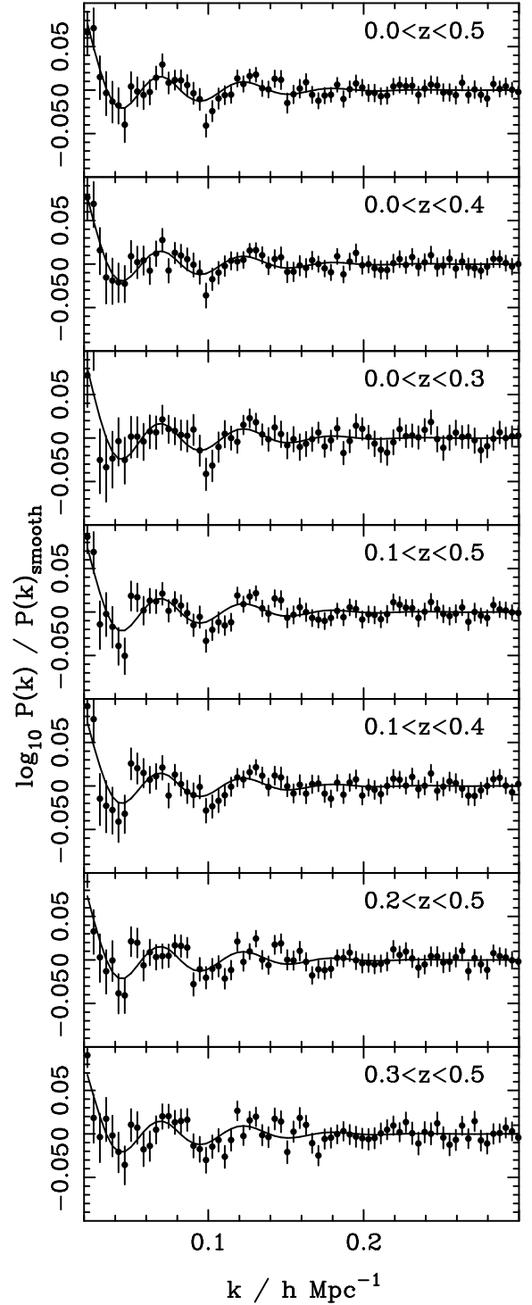
Figure 3. BAO recovered from the data for each of the redshifts slices (solid circles with 1-\sigma errors). These are compared with BAO in our default \Lambda\text{CDM} model (solid lines).
