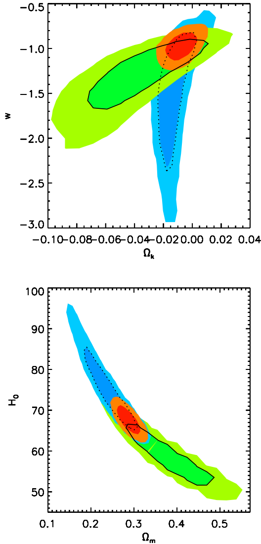
Figure 13. For the \omega wCDM model we compare the constraints from WMAP5+BAO (blue contours), WMAP5+SN (green contours), and WMAP5+BAO+SN (red contours). Dashed and solid contours highlight the 68% confidence intervals for the WMAP5+BAO and WMAP5+SN models respectively.
