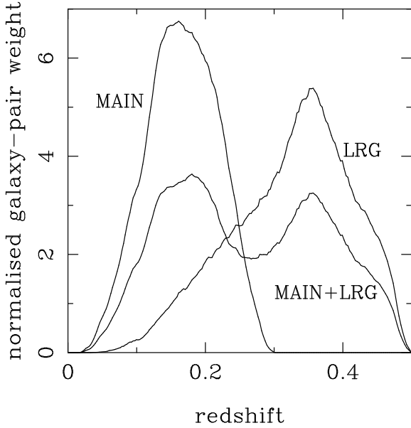
Figure A1. The redshift dependence of galaxy pair-weights for the SDSS DR7 LRG and main galaxy samples, and from the combination of the two. These curves were calculated assuming a flat \Lambda CDM cosmology with \Omega_m = 0.25 , h = 0.72 , & \Omega_b h^2 = 0.0223 .
