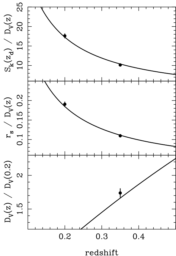
Figure 11. The BAO constraints (solid circles with 1\sigma errors), compared with the best-fit \Lambda CDM model. The three panels show different methods of using the data to constrain models.
