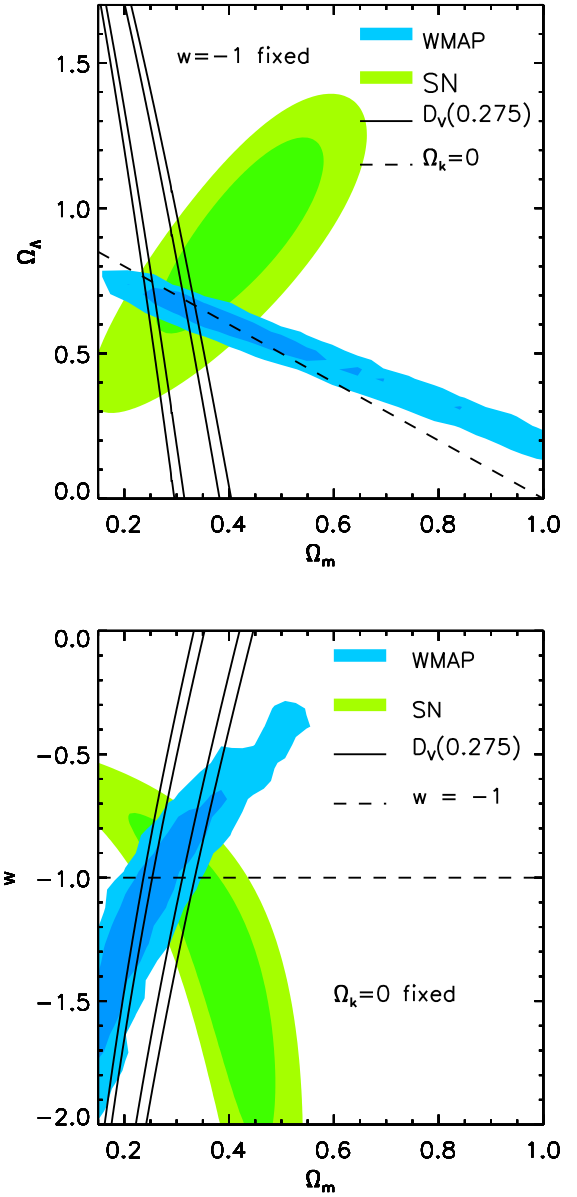
Figure 5. Cosmological constraints on \Lambda CDM cosmologies (upper panel) and flat CDM models where we allow w to vary (lower panel), from WMAP5 (blue), Union supernova (green) and our constraint on r_s/D_V(0.275) (solid contours). Contours are plotted for -2 \ln \mathcal{L}/\mathcal{L}_{\text{true}} < 2.3, 6.0 , corresponding to 68% and 95% confidence intervals. The dashed lines show flat models (upper panel) and \Lambda models (lower panel).
