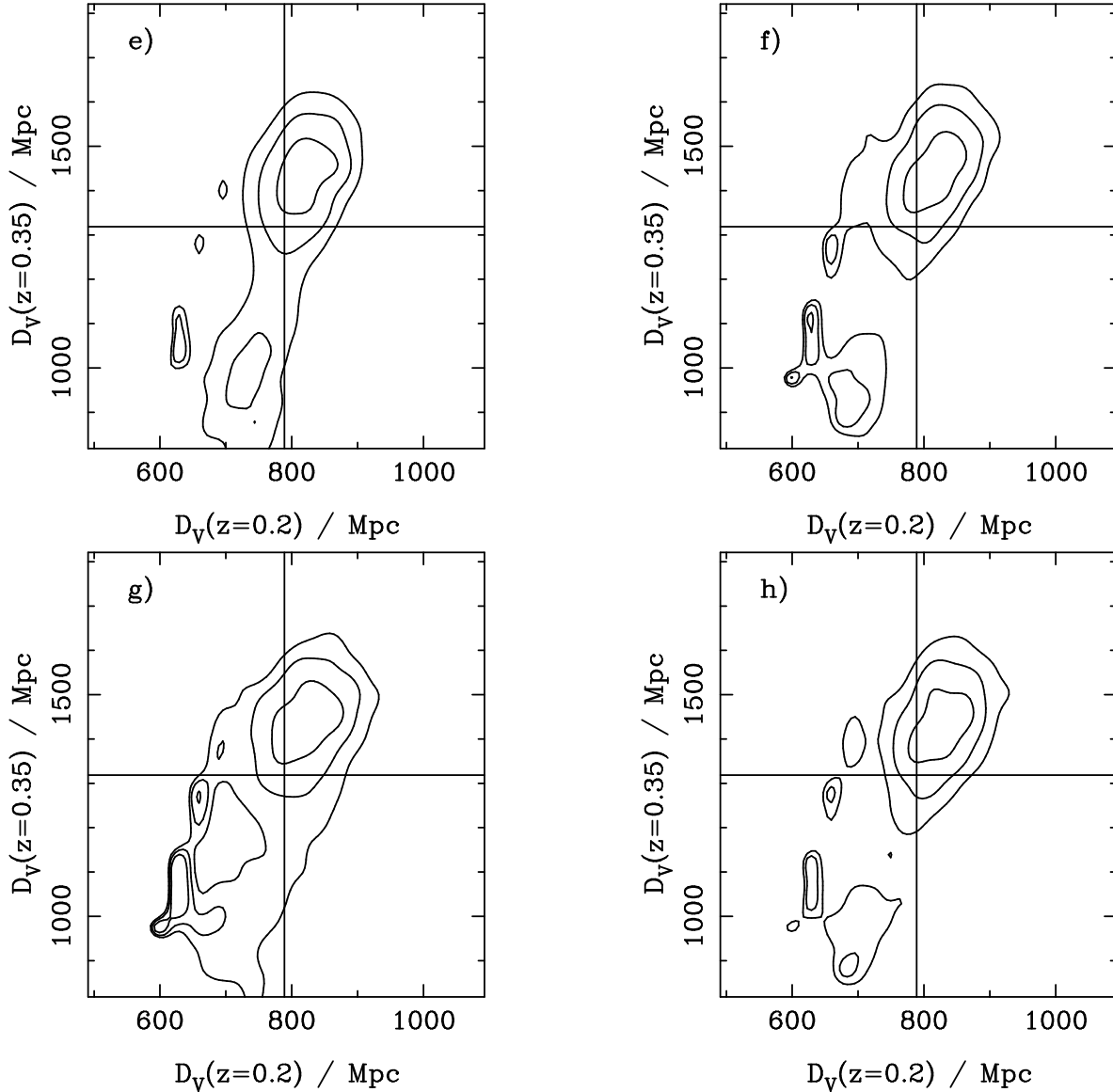
Figure 8. Likelihood contour plots as in Fig. 4, for the SDSS data, excluding the early data and the 2dFGRS, but now calculated for (e) fit to three power spectra, (f) old rather than uber-calibration. (g) allowing the BAO damping scale to vary with a simple Gaussian prior D_{\text{damp}} = 10 \pm 5 h^{-1} \text{ Mpc} , (h) randomized galaxy redshifts used to give the expected radial galaxy distribution.
