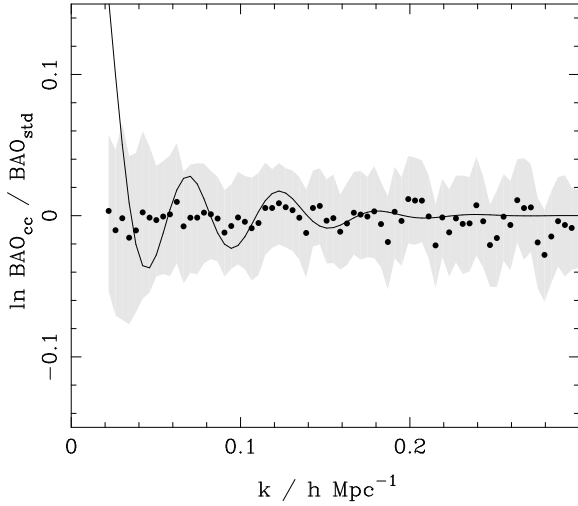
Figure 6. The log ratio between the BAO recovered from the SDSS LRG power spectrum and the power spectrum of the halo catalogue derived from the LRG sample as described by Reid et al. (2009) (solid circles). For comparison we plot the BAO expected for a flat \Lambda CDM model with \Omega_m = 0.25 , h = 0.72 , & \Omega_b h^2 = 0.0223 (solid line), and the errors on each measurement (grey shaded region). There are no oscillatory features induced by the cluster-collapse procedure, and the scatter is well within the errors.
