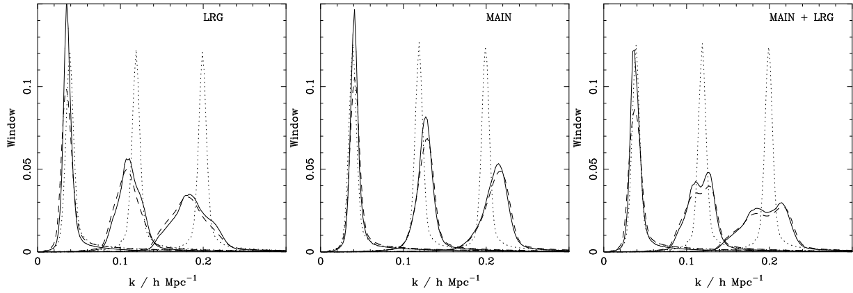
Figure A3. Window functions for three values of k , calculated for the SDSS LRG, main galaxy and combined catalogues. Dotted lines represent the windows for our fiducial \Lambda CDM cosmology. Solid and dashed lines show the window functions, if the true cosmology were different, but the data were analysed assuming that the fiducial \Lambda CDM cosmology is correct. The solid lines were calculated using the procedure outlined in this Appendix. Dashed lines were calculated using the Monte-Carlo procedure of Percival et al. (2007c).
