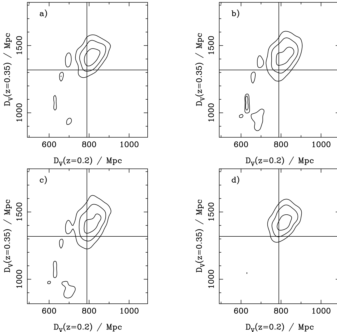
Figure 7. As Fig. 4, but now considering results from 4 choices of catalogue: (a) all SDSS and non-overlapping 2dFGRS data, (b) excluding both the early SDSS data and 2dFGRS, (c) excluding the 2dFGRS, (d) excluding the early SDSS data.
