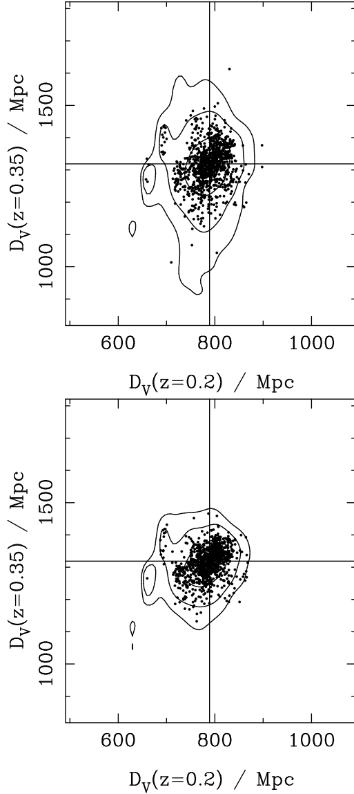
Figure 2. Average likelihood contours recovered from the analysis of three power spectra (top panel) and six power spectra (bottom panel) measured from 1000 Log-Normal density fields. Contours are plotted for -2 \ln \mathcal{L} = 2.3, 6.0, 9.2 , corresponding to two-parameter confidence of 68%, 95% and 99% for a Gaussian distribution. Contours were calculated after increasing the errors on the power spectrum band-powers as described in the text. Solid circles mark the locations of the likelihood maxima closest to the true cosmology. We have plotted the likelihood surface as a function of D_V(z)/\text{Mpc} , for fixed r_s(z_d) = 154.7 \text{ Mpc} , to show distance errors if the comoving sound horizon is known perfectly. The values of D_V for our input cosmology are shown by the vertical and horizontal solid lines.
