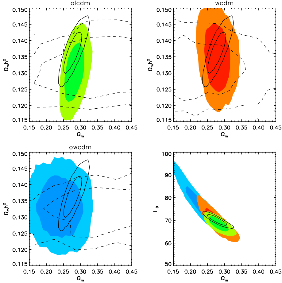
Figure 12. WMAP5+BAO constraints on \Omega_m h^2 , \Omega_m , and H_0 for \Lambda CDM (solid black contours), o\Lambda CDM (shaded green contours), w CDM (shaded red contours), and ow CDM (shaded blue contours) models. Throughout, the solid contours show WMAP5+LRG \Lambda CDM constraints. The first three panels show WMAP5 only constraints (dashed contours) and WMAP5+BAO constraints (colored contours) in the \Omega_m h^2 - \Omega_m plane as the model is varied. In the lower right we show all constraints from WMAP5+BAO for all four models in the \Omega_m - H_0 plane, which lie within the tight \Omega_m h^2 \approx 0.133 \pm 0.006 WMAP5-only constraints.
